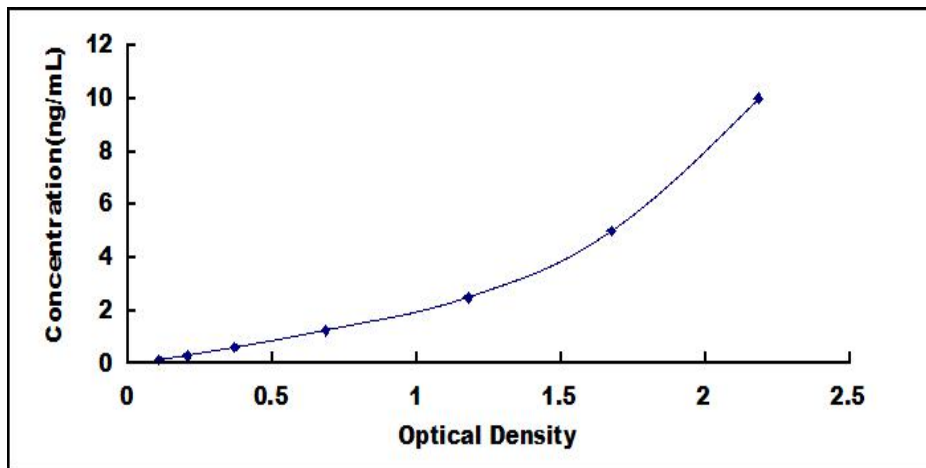
Typical Standard Curve for GZMK ELISA.
