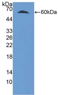
Figure 1. Western Blot
