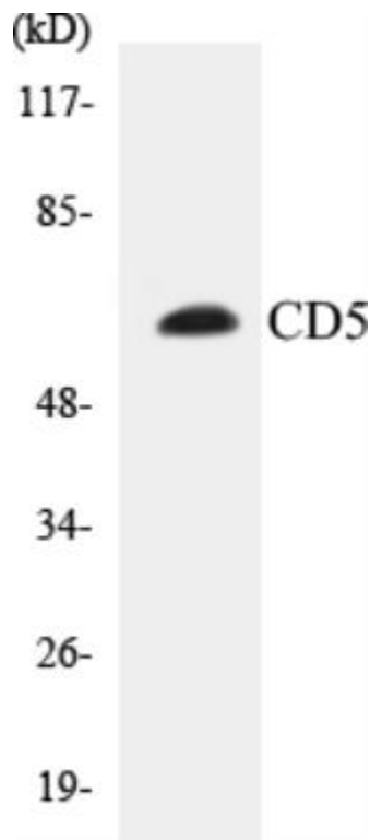
Figure 2. Western blot analysis of extracts from 293 cells, treated with PMA 125ng/ml 30' , using CD5 (Ab-Tyr453) Antibody.
