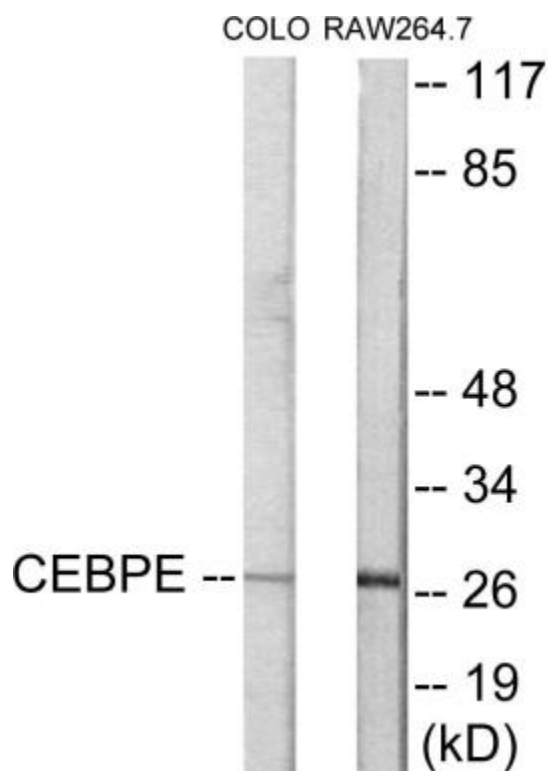
Figure 2. Western blot analysis of extracts from LOVO/RAW264.7 cells, using CEBPD/E Antibody. The lane on the right is treated with the synthesized peptide.
