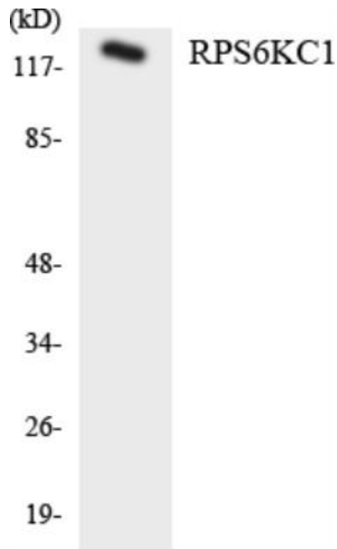
Figure 2. Western blot analysis of extracts from K562 cells, using RPS6KC1 Antibody.
