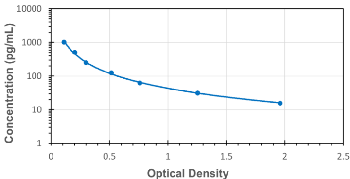
Typical Standard Curve for Rat CGRP ELISA
