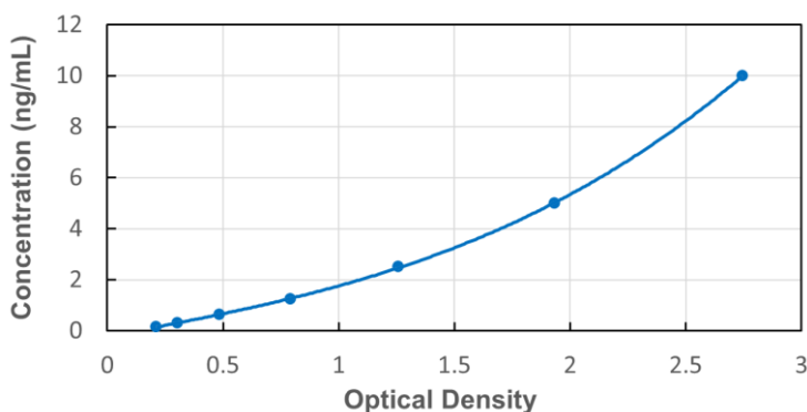
Typical Standard Curve for Rat CPB1 ELISA
