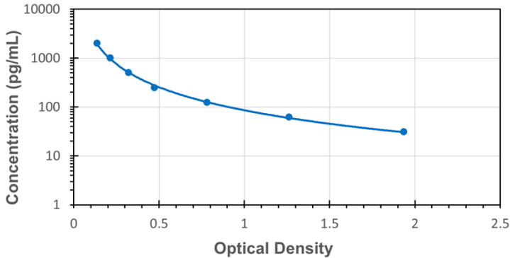
Typical Standard Curve for Human EDN2 ELISA
