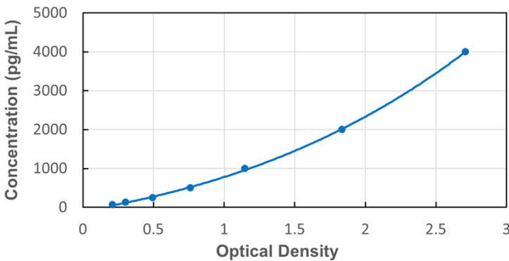
Typical Standard Curve for Rat EPO ELISA
