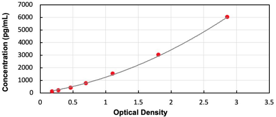
Typical Standard Curve for Mouse IGF2 ELISA
