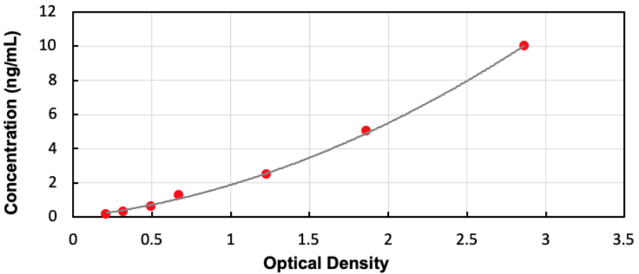
Typical Standard Curve for Mouse IL11Ra ELISA
