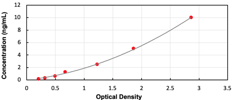
Typical Standard Curve for Human IL18RAP ELISA
