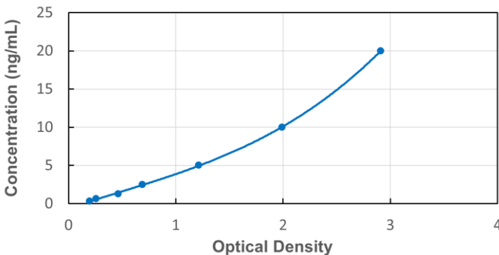
Typical Standard Curve for Human PSMD3 ELISA
