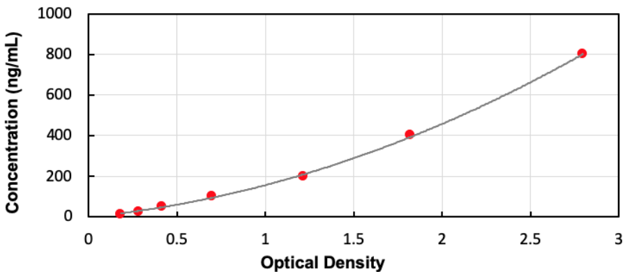
Typical Standard Curve for Human AFM ELISA
