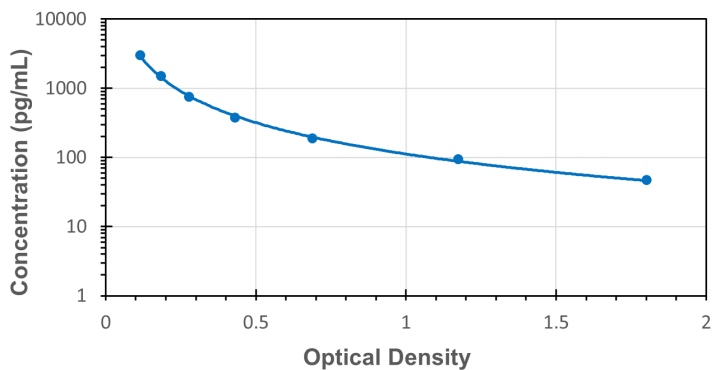
Typical Standard Curve for Human AMH ELISA
