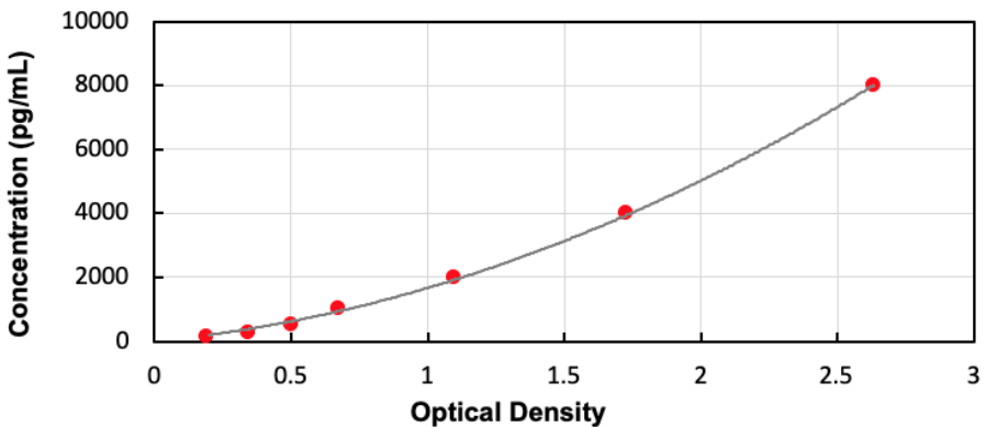
Typical Standard Curve for Human bTG ELISA
