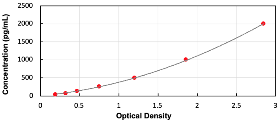
Typical Standard Curve for Human CCBE1 ELISA
