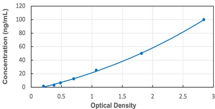
Typical Standard Curve for Human CFP ELISA
