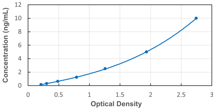
Typical Standard Curve for Human CPB1 ELISA
