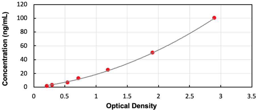
Typical Standard Curve for Human CSE ELISA
