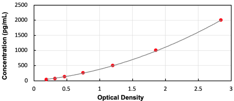
Typical Standard Curve for Human EPCAM ELISA
