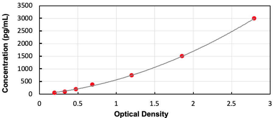
Typical Standard Curve for Human FGL2 ELISA
