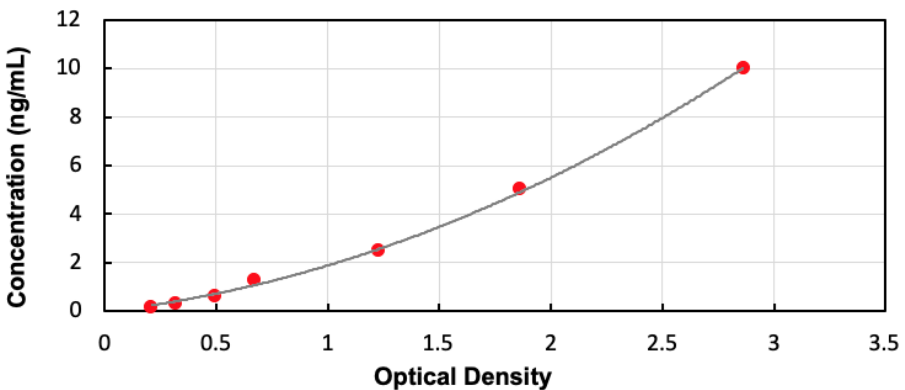
Typical Standard Curve for Human GDF5 ELISA
