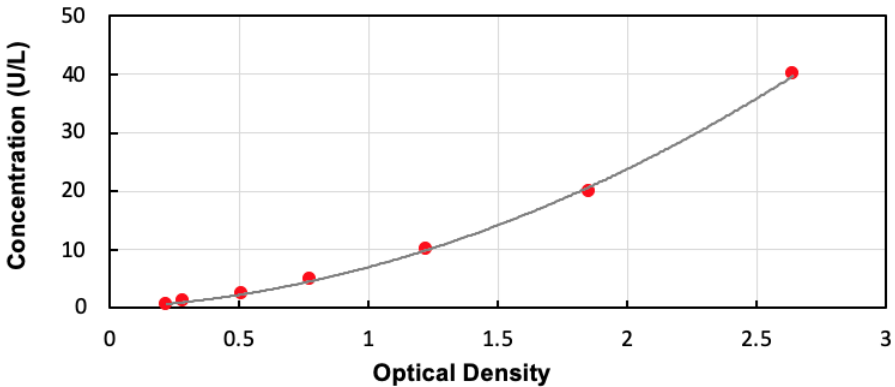
Typical Standard Curve for Human GDH ELISA
