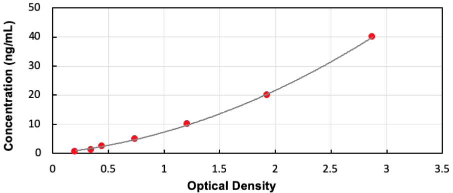
Typical Standard Curve for Human GPR120 ELISA
