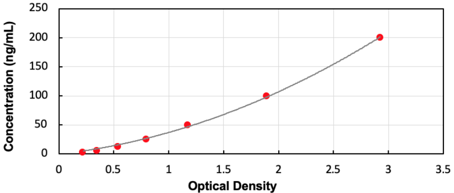
Typical Standard Curve for Human HAase ELISA
