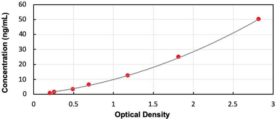
Typical Standard Curve for Human HMGCR ELISA
