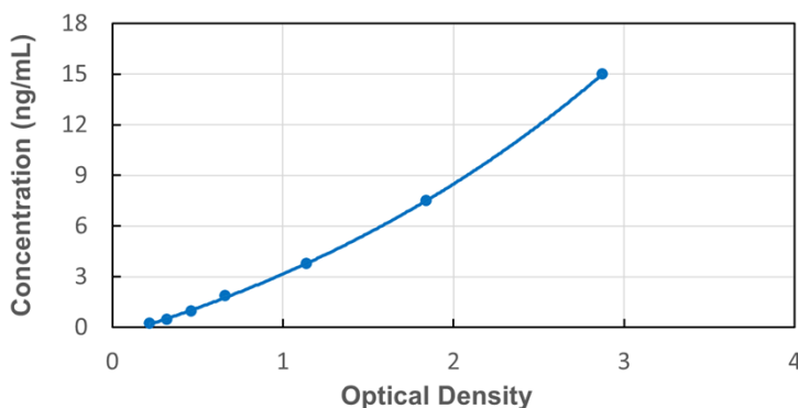
Typical Standard Curve for Human LECT2-Hu ELISA
