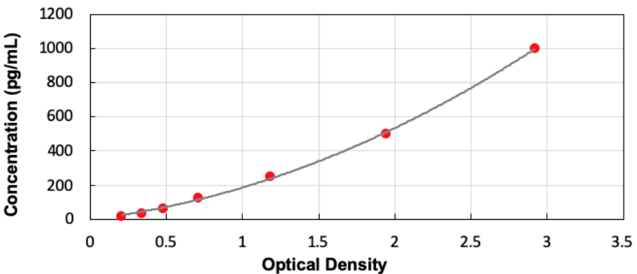
Typical Standard Curve for Human METRN ELISA
