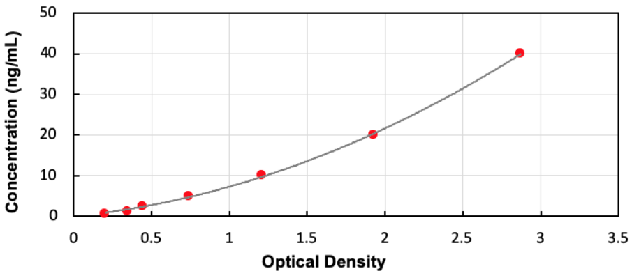
Typical Standard Curve for Human MPP2 ELISA
