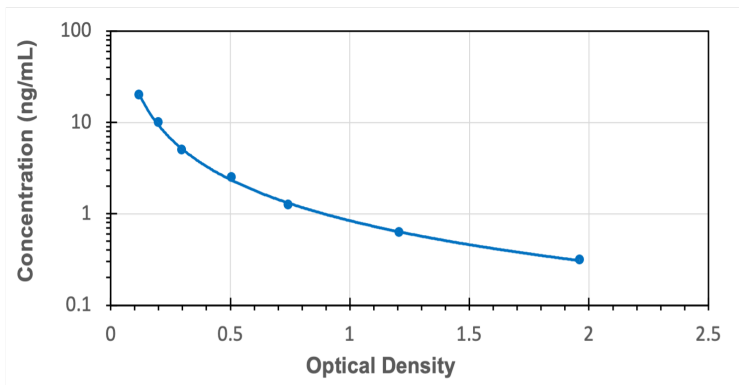
Typical Standard Curve for Human NUDT11 ELISA
