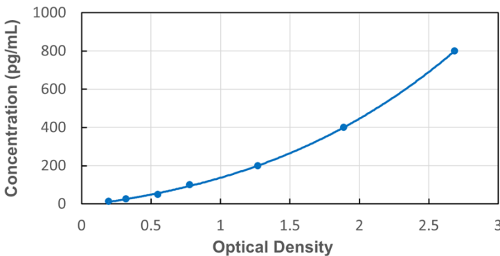
Typical Standard Curve for Human PIIICP ELISA
