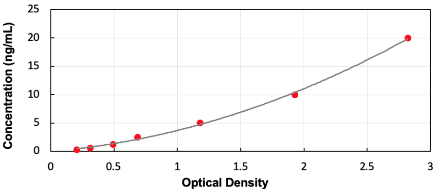
Typical Standard Curve for Human SAA ELISA
