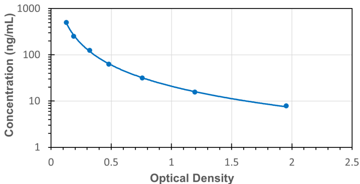
Typical Standard Curve for Human TMSb10 ELISA
