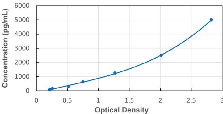
Typical Standard Curve for Human TSHR ELISA
