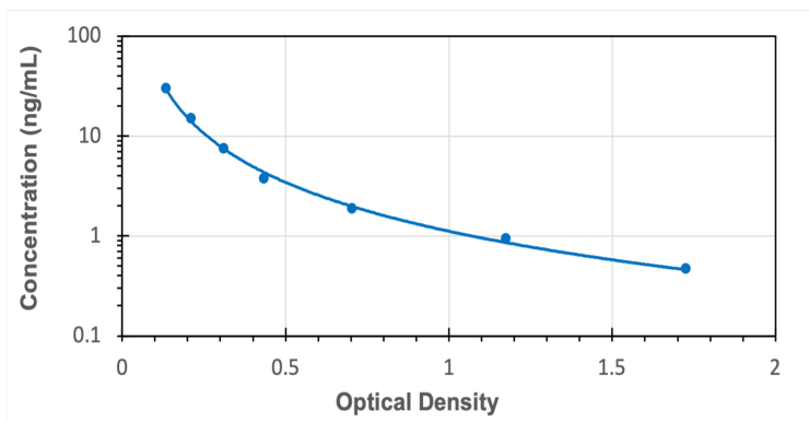
Typical Standard Curve for Rat LH ELISA
