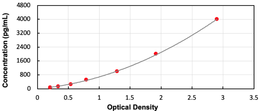
Typical Standard Curve for Mouse OC ELISA
