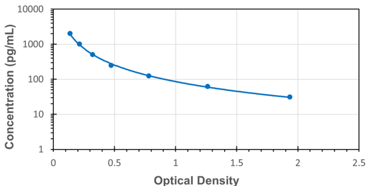
Typical Standard Curve for General BK ELISA
