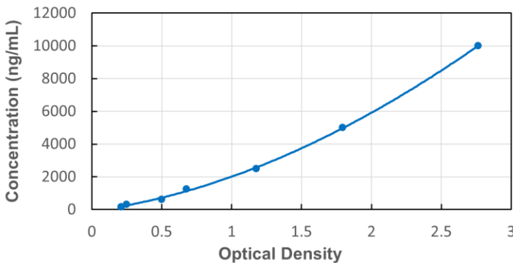
Typical Standard Curve for Rat LDL ELISA
