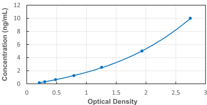
Typical Standard Curve for Human OPG ELISA
