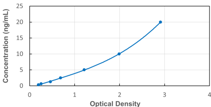
Typical Standard Curve for Mouse LPCAT2 ELISA
