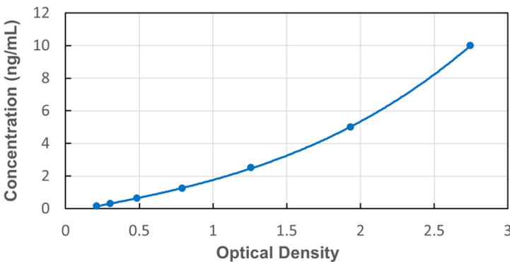
Typical Standard Curve for Mouse ASS1 ELISA
