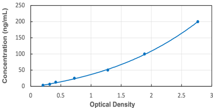
Typical Standard Curve for Rat PON1 ELISA
