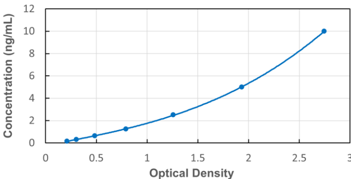
Typical Standard Curve for Mouse FABP2 ELISA
