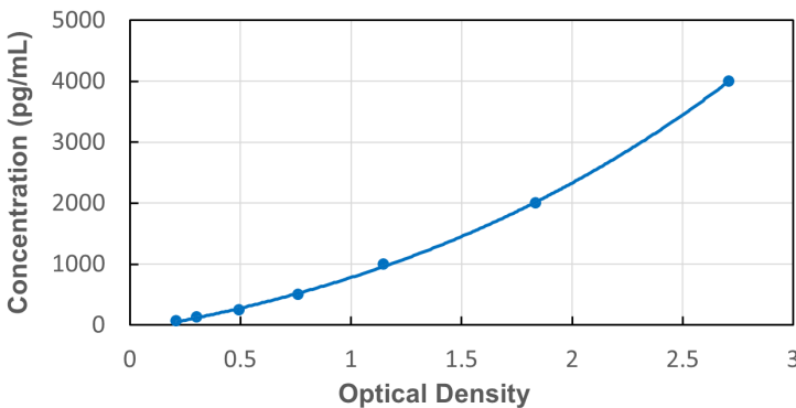
Typical Standard Curve for Human CNP ELISA
