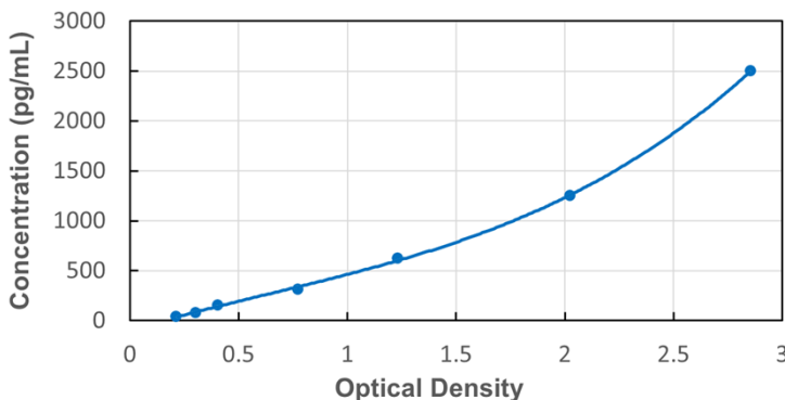
Typical Standard Curve for Human GPX1 ELISA
