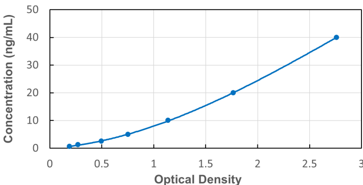
Typical Standard Curve for Human GSTa1 ELISA
