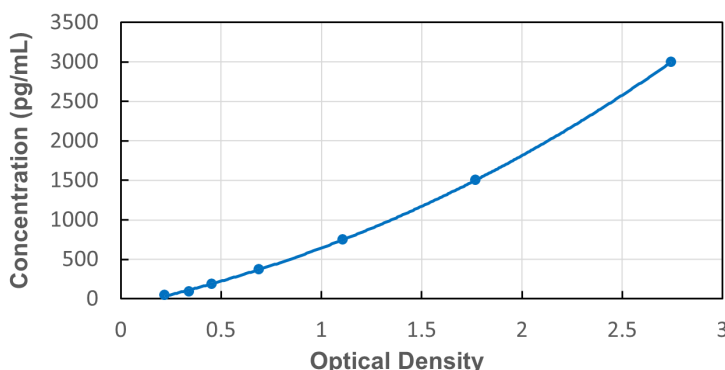
Typical Standard Curve for Human FcγRII ELISA
