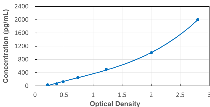
Typical Standard Curve for Human HTRA1 ELISA
