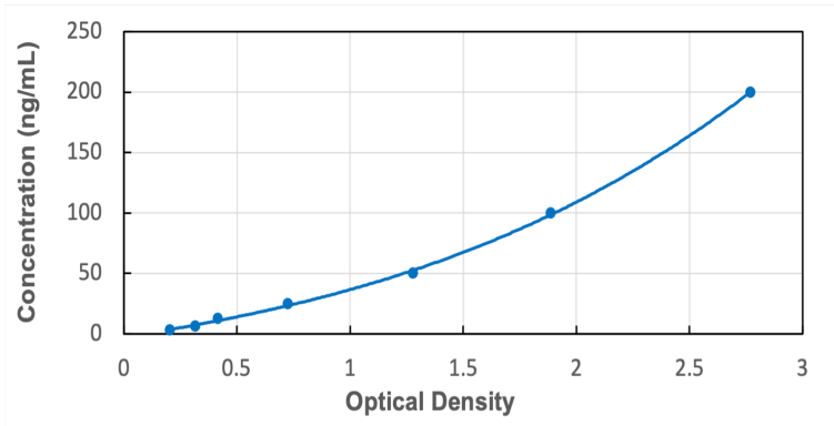
Typical Standard Curve for Mouse APOB ELISA
